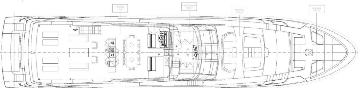
FLY DECK
