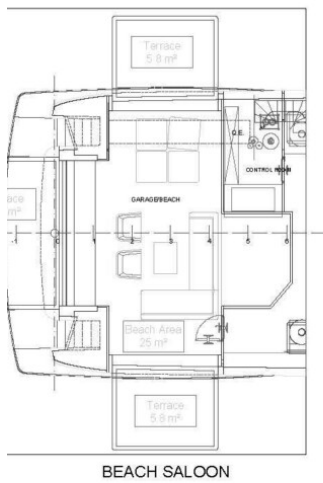
BEACH SALOON
