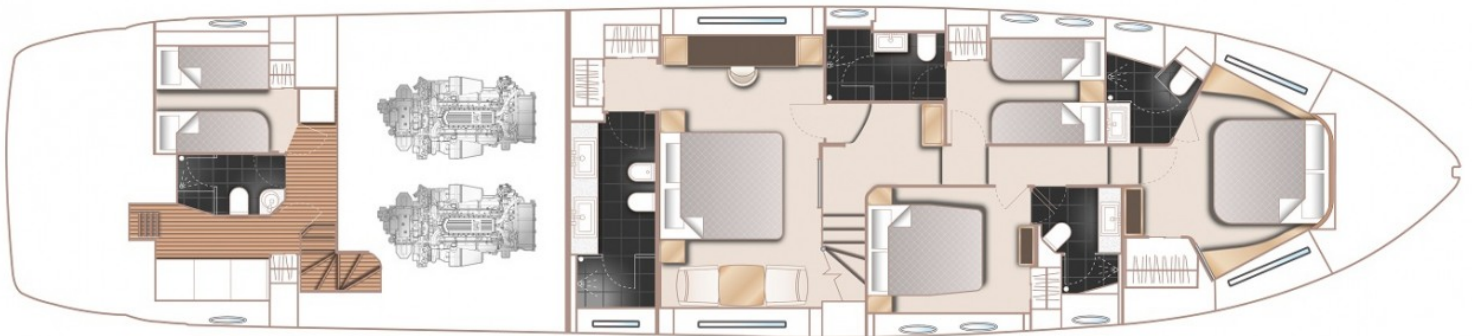
LOWER DECK
