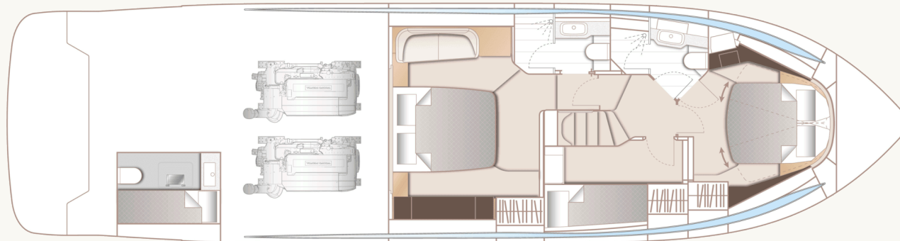
V55 Lower Deck
