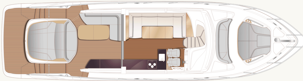
V55 Main Deck
