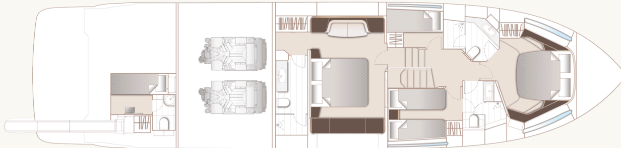
V65 Main Deck
