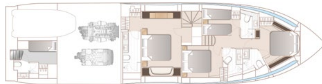
LOWER DECK
