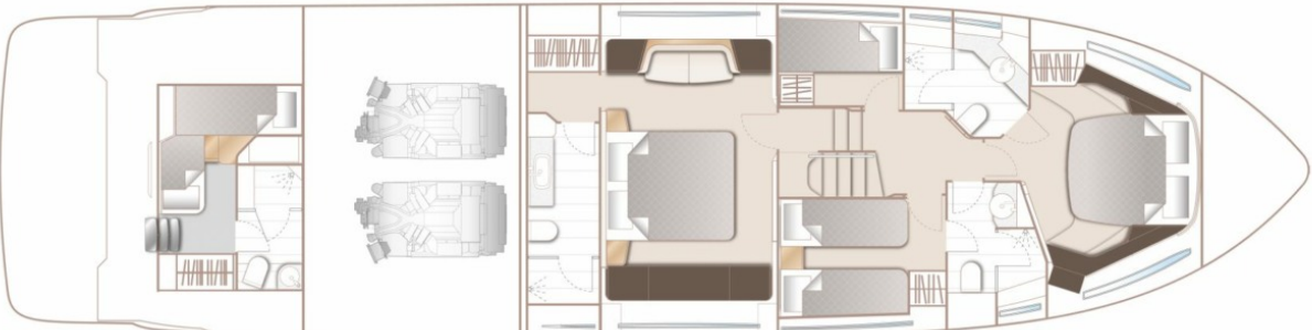
LOWER DECK
